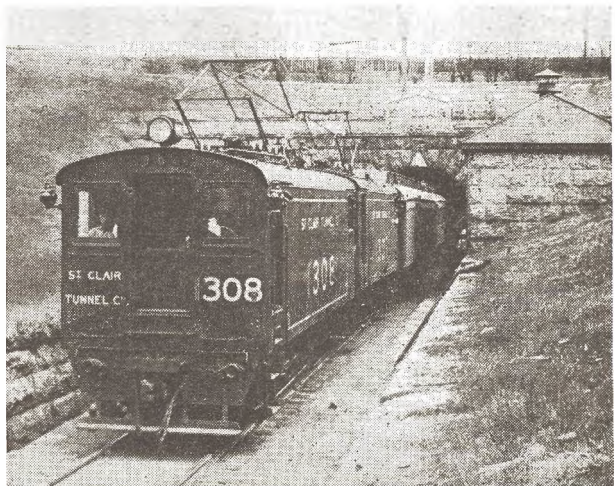
THIRTY-THREE HUNDRED volt a.c. motors have been growling through the bore between Port Huron, Mich., and Sarnia, Ont., since 1908. This is the only railroad tunnel crossing the international boundary line
