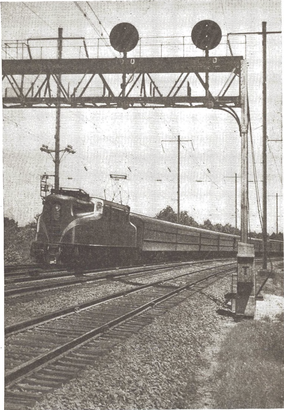
BETWEEN Potomac Yards and Sunny Side, L. I., gold-stripped, P-5As and Raymond Loewy-contoured GG-1s touch their pantographs to catenarys strung under 855 miles of heavy transmission cable sheaved to more than 8000 five-ton steel poles. At left: The 4920 leaving Washington terminal with a passenger train. Above: GG-1 southbound passes under a signal tower
