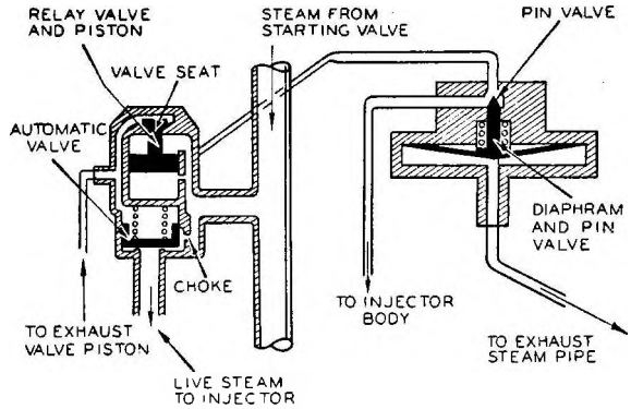
PRINCIPLE of exhaust steam injector change-over
